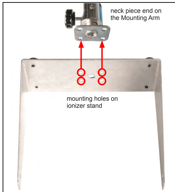
Figure 3. Installing the ionizer's stand to the Ionizer Mounting Arm
