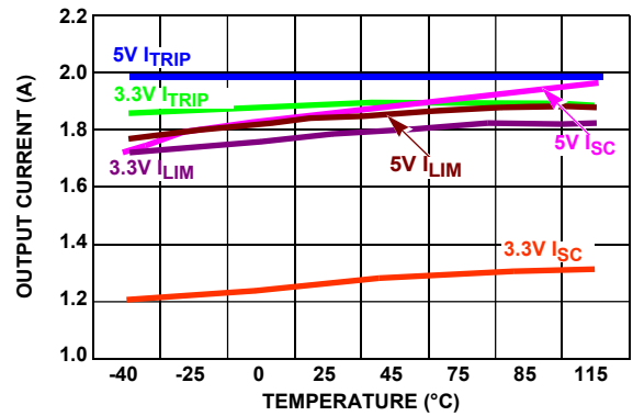
FIGURE 8. 1.8A CONTINUOUS CURRENT CHARACTERISTICS
