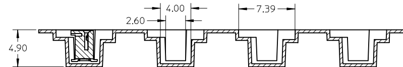
SECTION Z-Z
