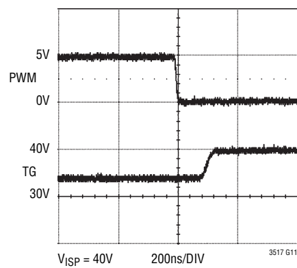
PMOS Turn-Off
