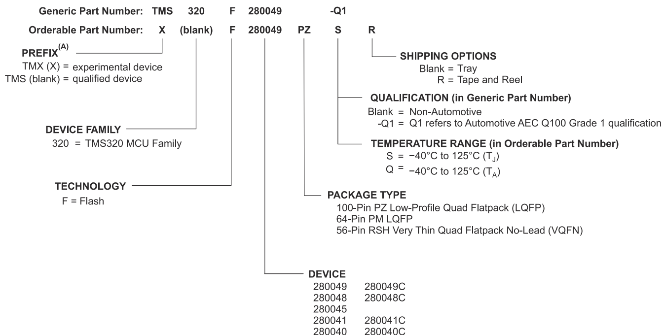
Figure 10-1. Device Nomenclature
