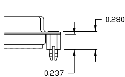
05X ..... 0.237" (BOARD SIDE) - CN10
