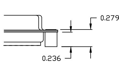
02X ..... 0.236" (BOARD SIDE) - CN2
