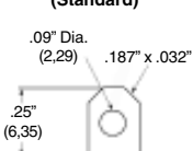
S 2 Solder Eye & Quick Connect (Standard)
