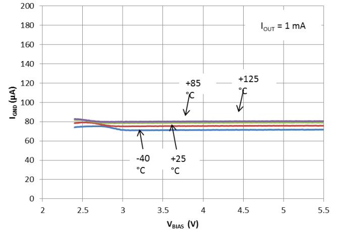
Figure 7. Bias Pin Current vs. V_{BIAS} Input Voltage
