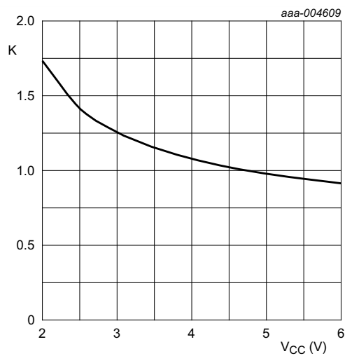
K-factor for 74HC1G14-Q100
