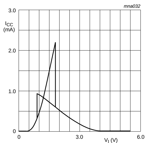
Fig 13. Typical 74HCT1G14-Q100 transfer characteristics; V_{CC} = 5.5\text{ V}
