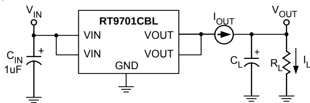
Test Circuit 1
