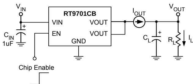
Test Circuit 3
