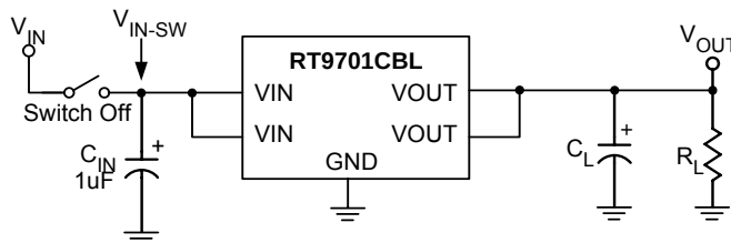
Test Circuit 2
