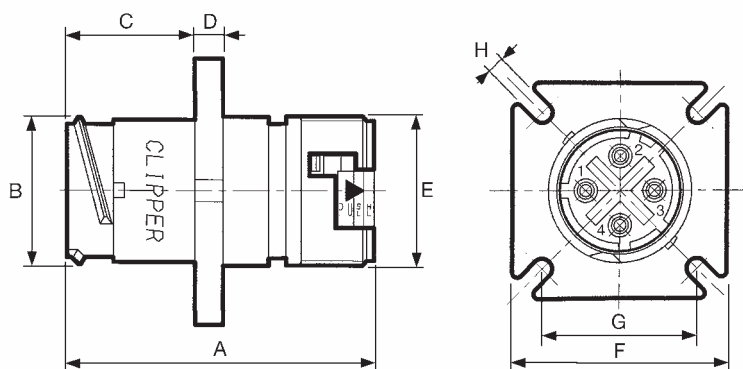
Square flange receptacle
