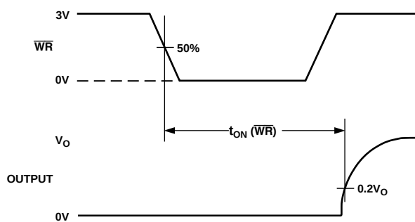
Test Circuit 8. Write Turn-On Time, t_{ON} (WR)
