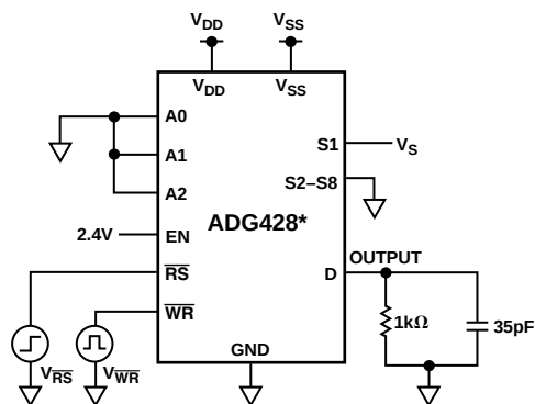
Test Circuit 8. Write Turn-On Time, t_{ON} (WR)
