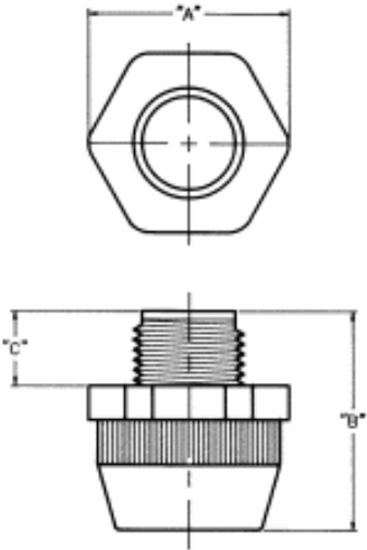
Straight Connector
