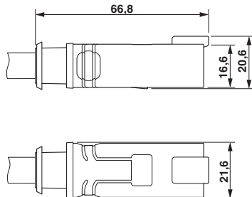
Dimensional drawing
