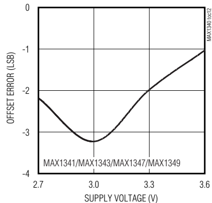
ADC OFFSET ERROR vs. ANALOG SUPPLY VOLTAGE
