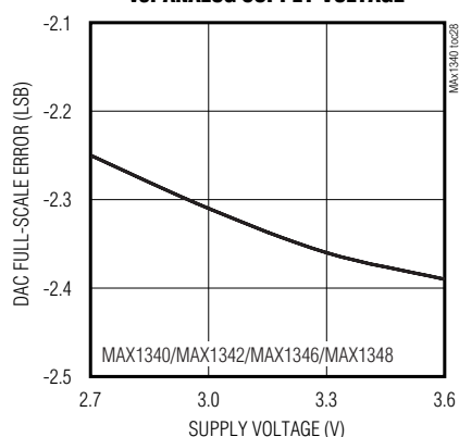
DAC FULL-SCALE ERROR vs. ANALOG SUPPLY VOLTAGE
