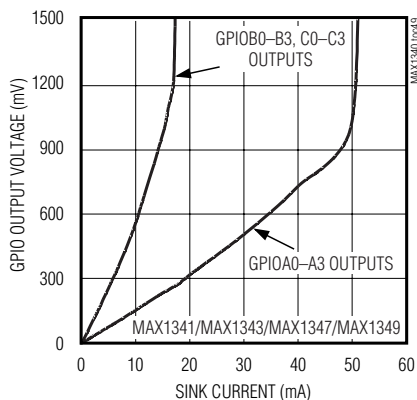
GPIO OUTPUT VOLTAGE vs. SINK CURRENT
