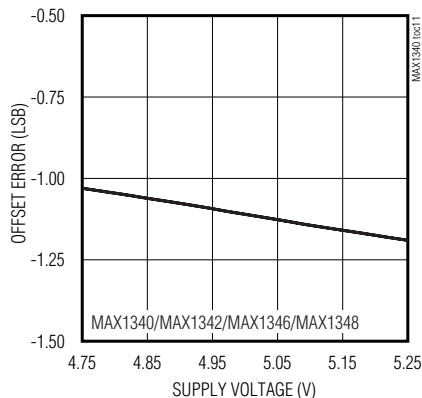
ADC OFFSET ERROR vs. ANALOG SUPPLY VOLTAGE
