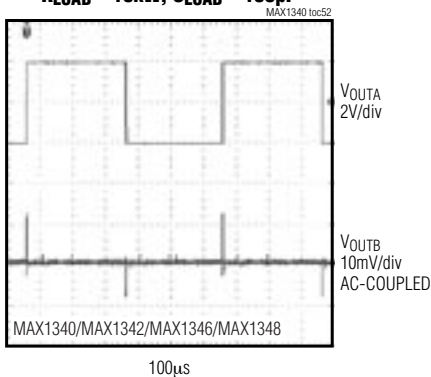
DAC-TO-DAC CROSSTALK R_{LOAD} = 10k\Omega , C_{LOAD} = 100pF
