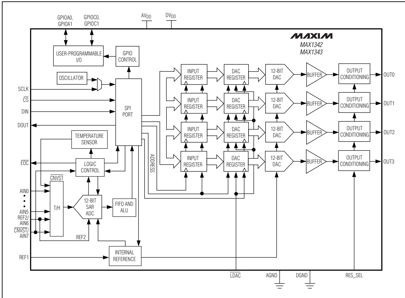
Figure 1. MAX1342/MAX1343 Functional Diagram
