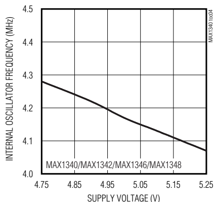
INTERNAL OSCILLATOR FREQUENCY vs. ANALOG SUPPLY VOLTAGE
