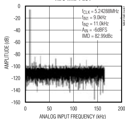
ADC IMD PLOT
