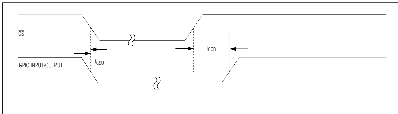
Figure 13. GPIO Timing
