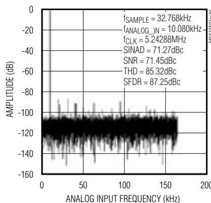
ADC FFT PLOT
