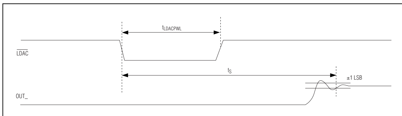
Figure 14. \overline{\text{LDAC}} Functionality
