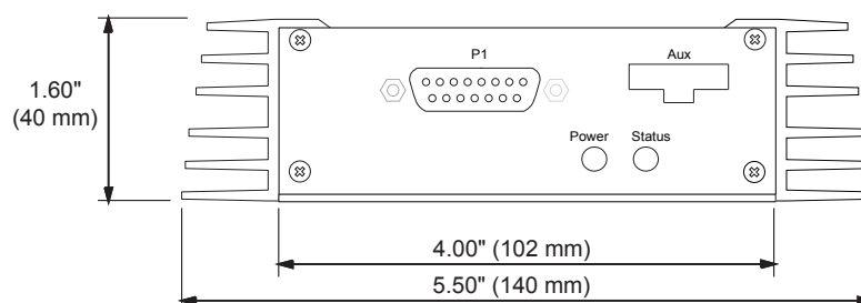
FIGURE 15. VDC2450 front view and dimensions
