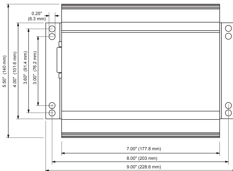
FIGURE 16. VDC2450 top view and dimensions
