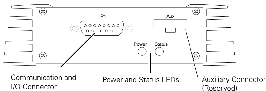
FIGURE 10. Front Controller Layout
