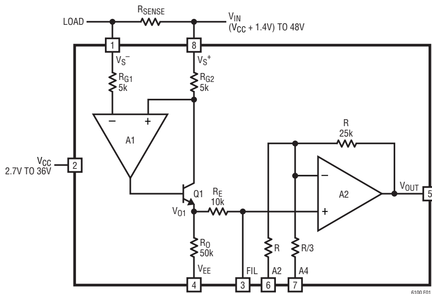
Figure 1. Functional Diagram
