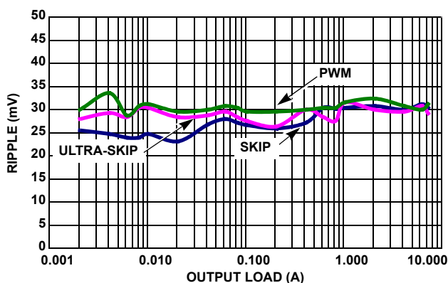
FIGURE 8. V_{OUT1} = 1.5V RIPPLE vs LOAD
