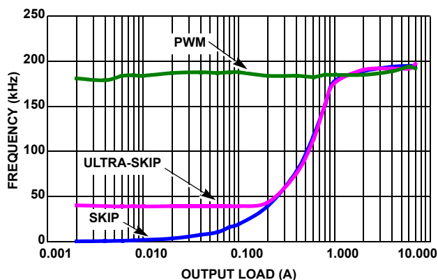
FIGURE 7. V_{OUT1} = 1.5V FREQUENCY vs LOAD
