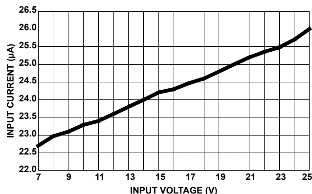
FIGURE 16. SHUTDOWN INPUT CURRENT vs V_{IN} ( EN = EN2 = EN\_LDO = 0 )
