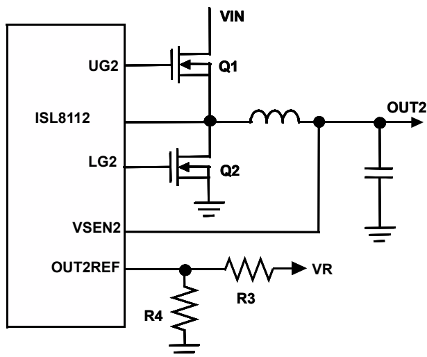
FIGURE 28. SETTING V_{OUT2} WITH A VOLTAGE DIVIDER FOR TRACKING
