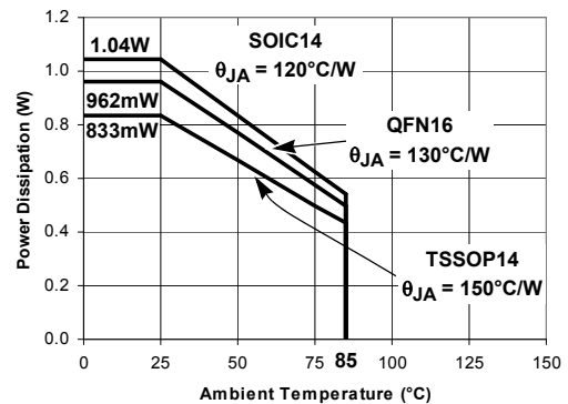
FIGURE 30. PACKAGE POWER DISSIPATION vs AMBIENT TEMPERATURE
