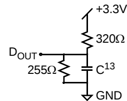
Figure B: 3.3V Output load
