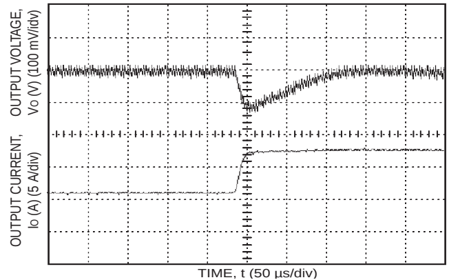
Figure 11. Transient Response to Step Increase in Load from 50% to 75% of Full Load ( V_I = 48 Vdc).
