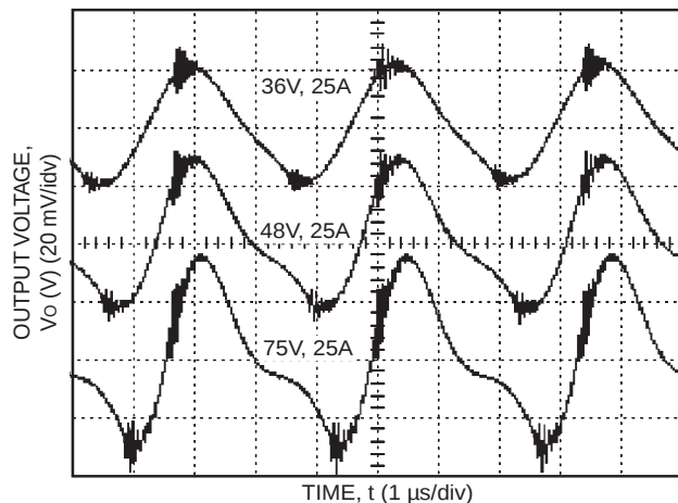
Figure 9. Output Ripple Voltage ( I_O = I_{O, \max} ).
