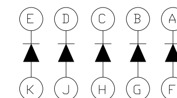
SCHEMATIC DIAGRAM
