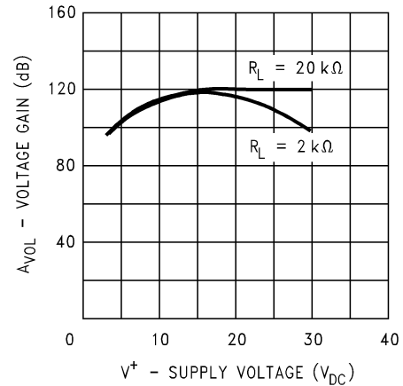
Figure 6-4. Voltage Gain
