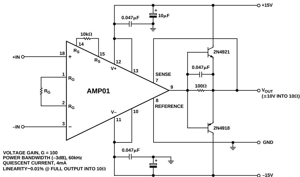
Figure 38. Adding Two Transistors Increases Output Current to \pm 1\text{ A} Without Affecting the Quiescent Current of 4 mA. Power Bandwidth is 60 kHz.
