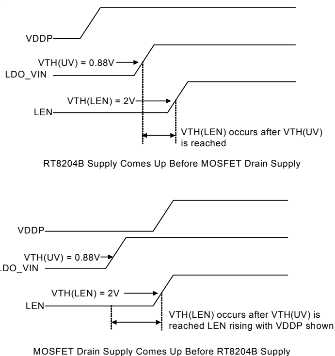
Figure 7. Power Supply Sequencing
