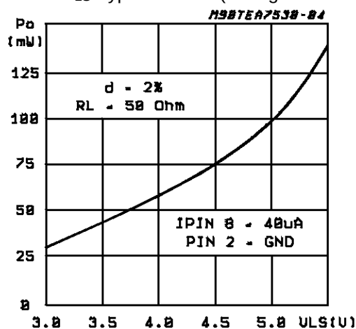
Figure 2: Power Available on Loudspeaker vs. V LS Typical Curve. (Voltage Mode)
