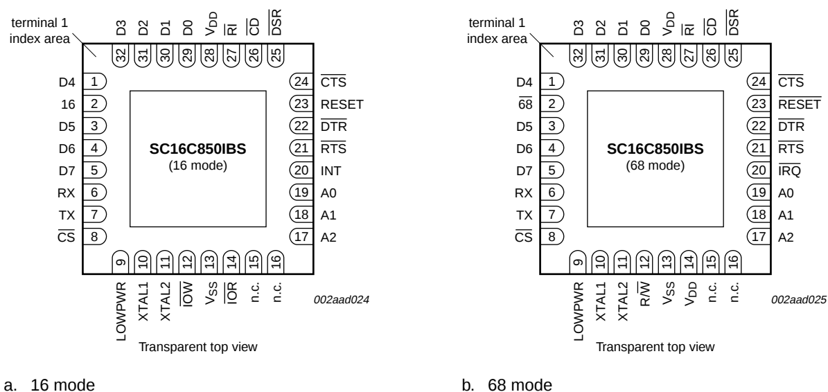
Fig 5. Pin configuration for HVQFN32
