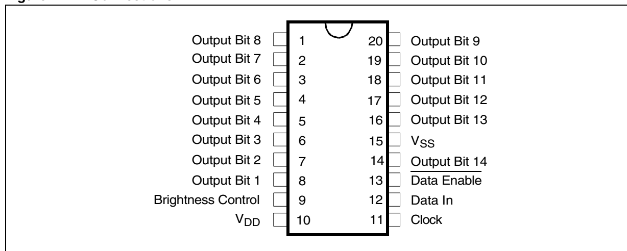
Figure 2. Pin Connections
