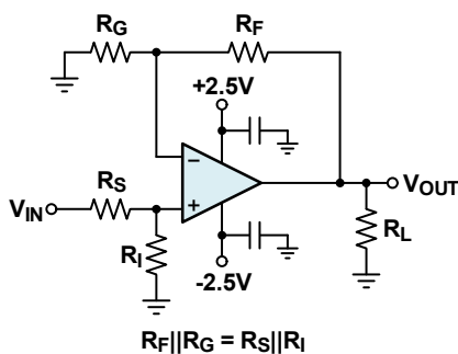
FIGURE 44. CIRCUIT IMPLEMENTATION FOR REDUCING INPUT BIAS CURRENTS
