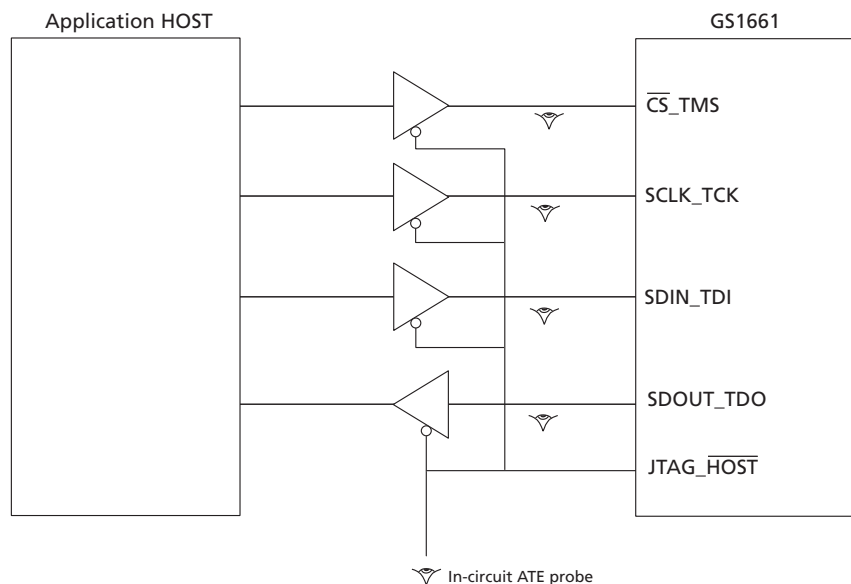
Figure 4-32: In-Circuit JTAG
