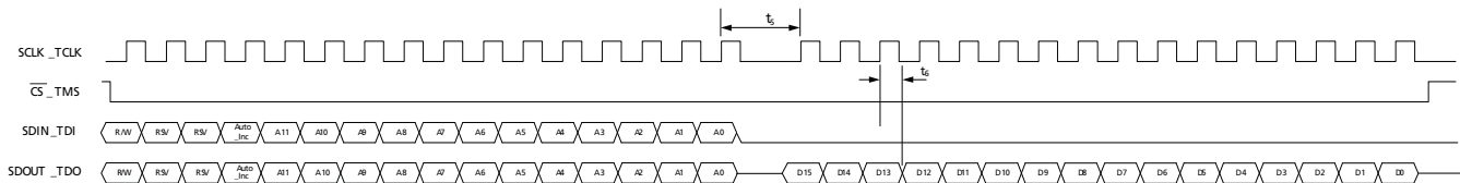
Figure 4-30: Read Mode
