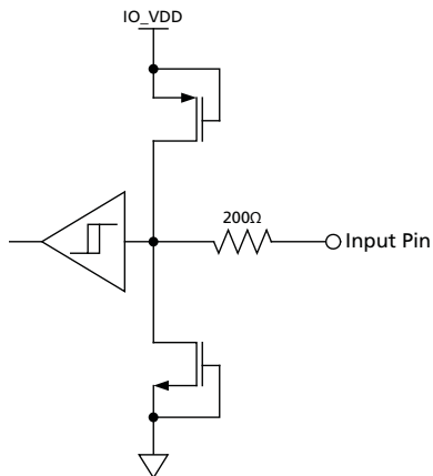
Figure 3-1: Digital Input Pin with Schmitt Trigger (20bit/10bit, \overline{\text{CS\_TMS}} , SW_EN, IOPROC_EN/ \overline{\text{DIS}} , JTAG/ \overline{\text{HOST}} , \overline{\text{RC\_BYP}} , \overline{\text{RESET\_TRST}} , SCLK_TCK, SDIN_TDI, SDO_EN/ \overline{\text{DIS}} , STANDBY, TIM_861)
