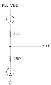
Figure 3-7: Loop Filter
