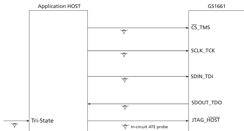
Figure 4-33: System JTAG
