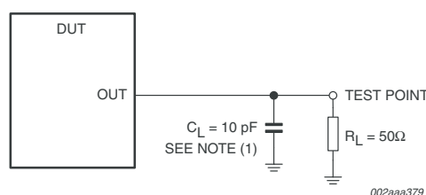
Figure 14 — Load circuit, LOW-to-HIGH slew measurement
