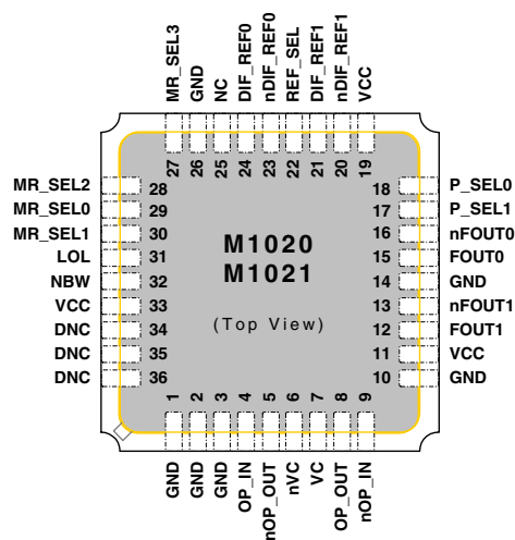
Figure 1: Pin Assignment
