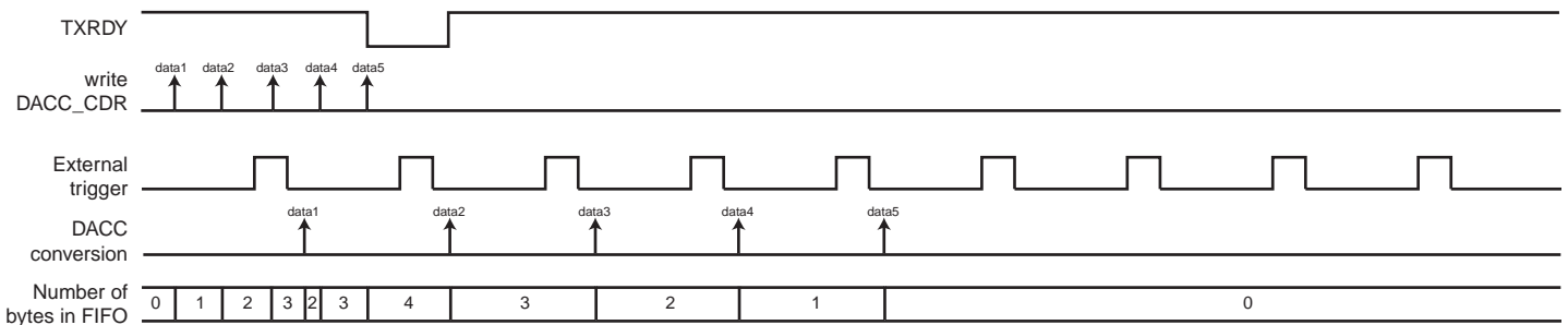
Figure 35-3. External trigger
