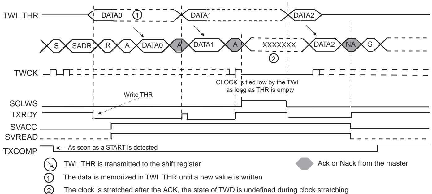
Figure 29-28. Clock Synchronization in Read Mode
