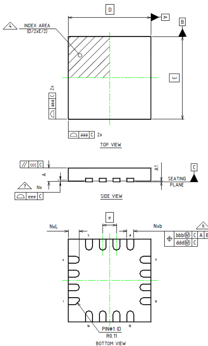
Figure 11. QFN 16 (3x3 mm) package outline
