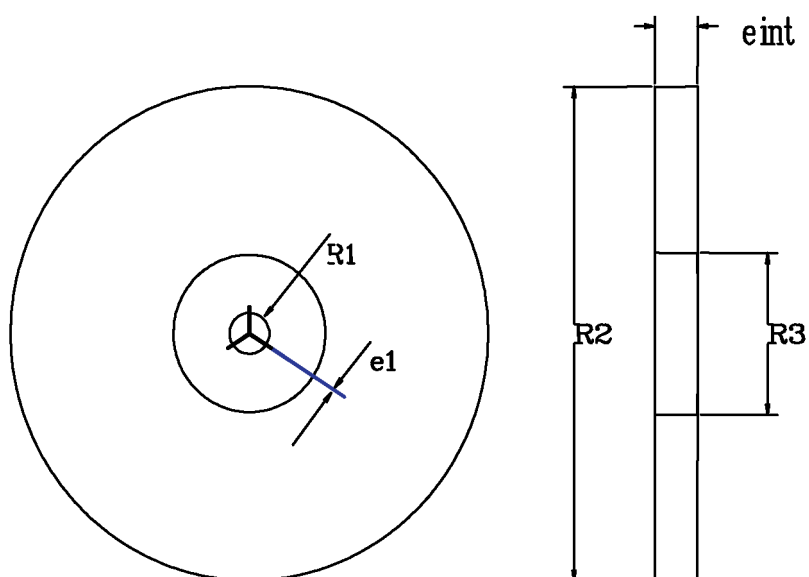
Figure 12. Reel information
