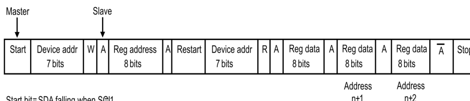
Figure 4. Read operation
