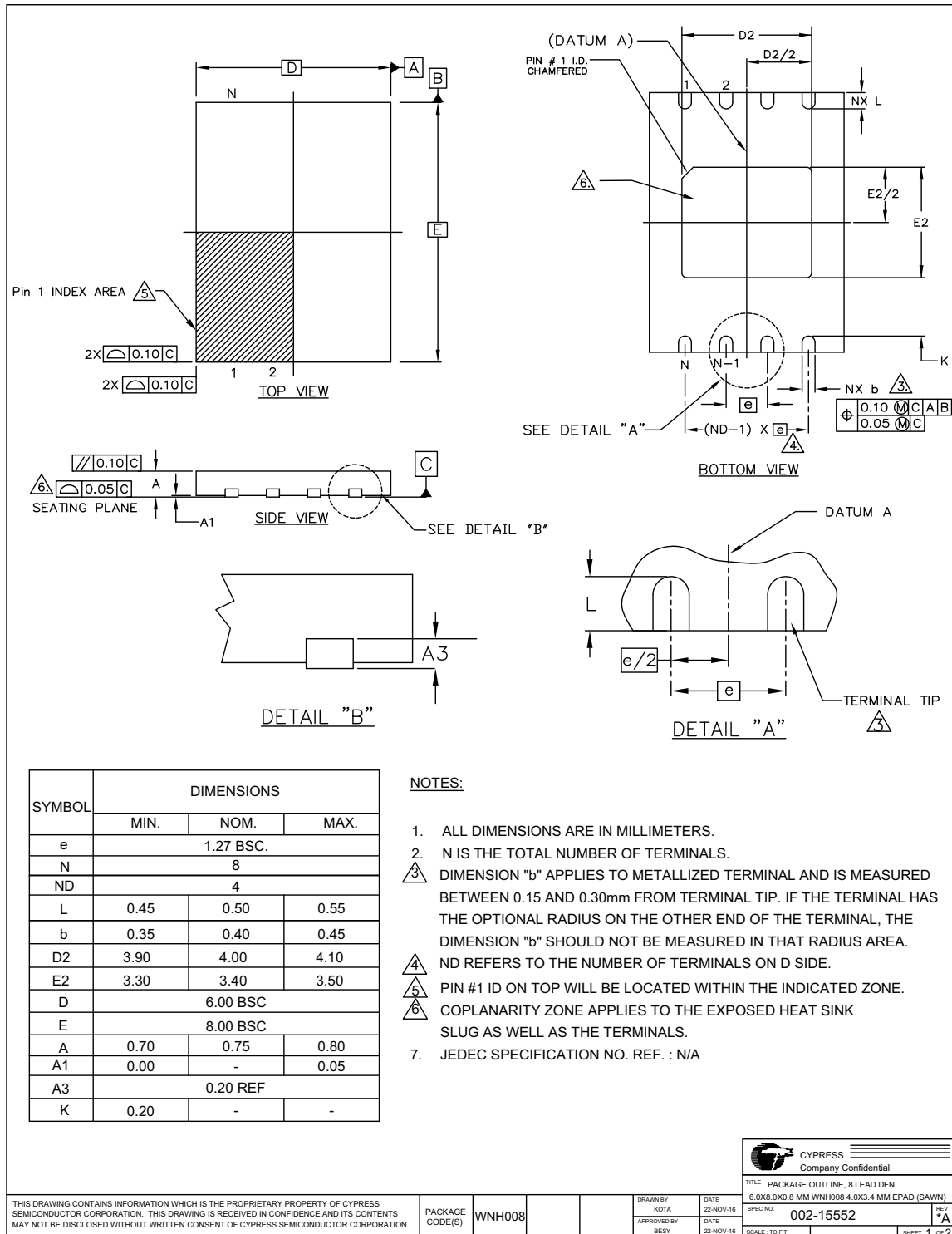
Figure 39. WSON 8-Contact 6x8 mm Leadless (WNH008)
