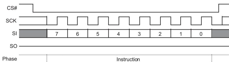
Figure 116. Deep Power-Down Command Sequence
