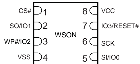
Figure 38. 8-Connector Package (WSO6 6x8), Top View
