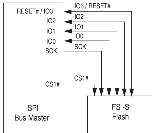
Figure 3. Bus Master and Memory Devices on the SPI Bus — Quad Bit Data Path
