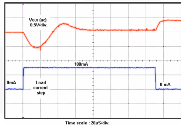
Figure 9. Load Transient Response
