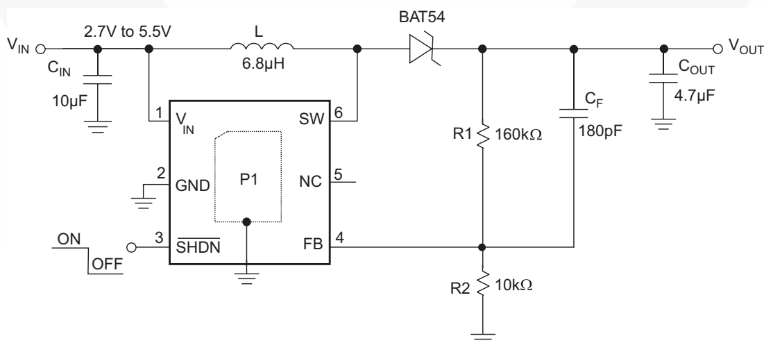
Figure 3. Test Circuit
