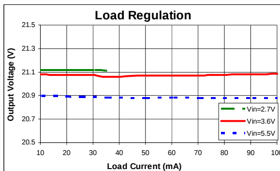
Figure 5. Load Regulation
