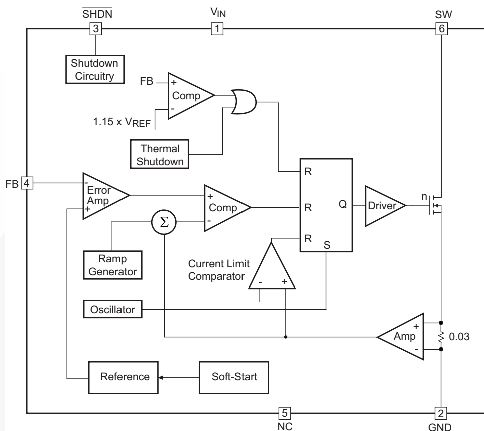
Figure 10. Block Diagram
