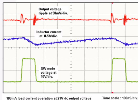
Figure 7. 100mA Load Current Operation
