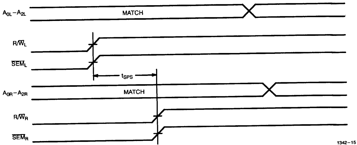
Timing Diagram of Semaphore Contention (CY7B1342 only) [22, 23, 24]
