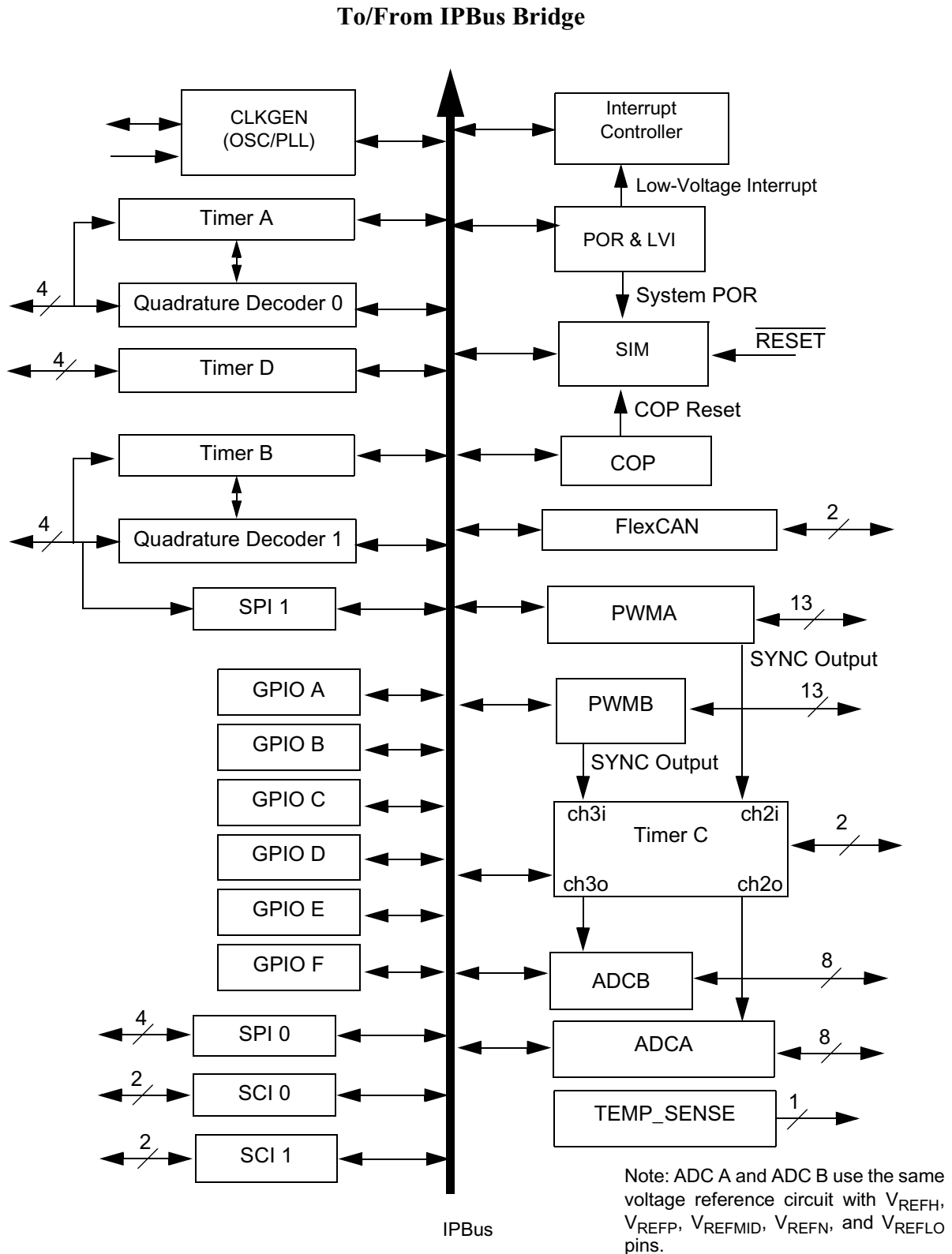
Figure 1-2 Peripheral Subsystem
