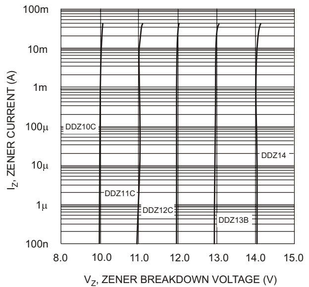
Fig. 5 Typical Reverse Characteristics, DDZ10C - DDZ14
