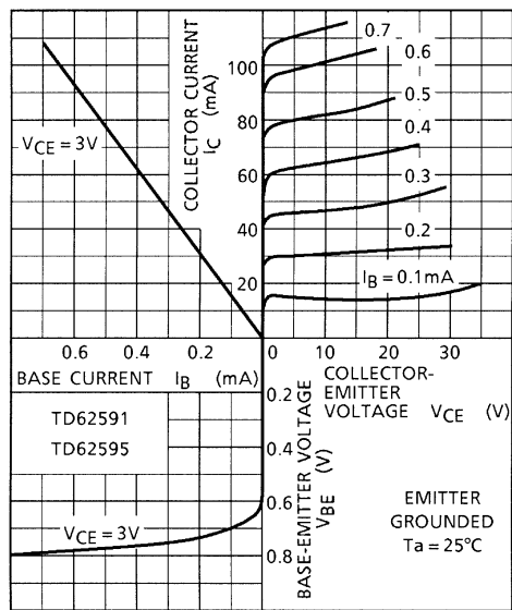
STATIC CHARACTERISTICS
