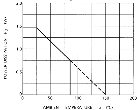
P_D - T_a
