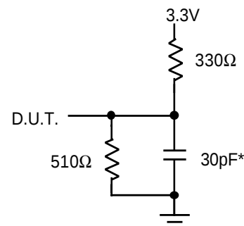
Figure 2. Output Load
