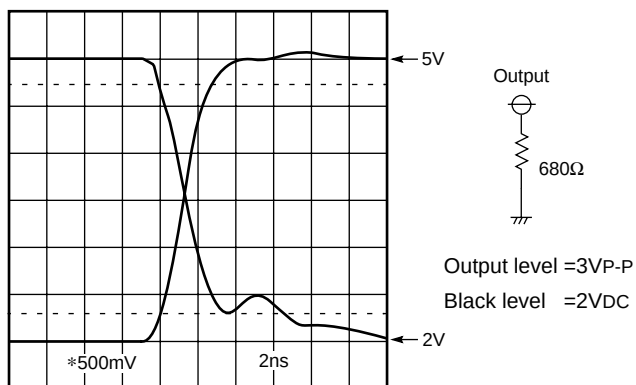
RISE AND FALL OF OUTPUT WAVEFORM (3VP-P)
