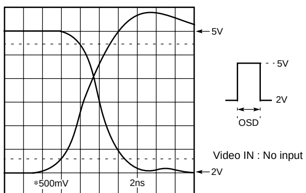
RISE AND FALL OF OSD
