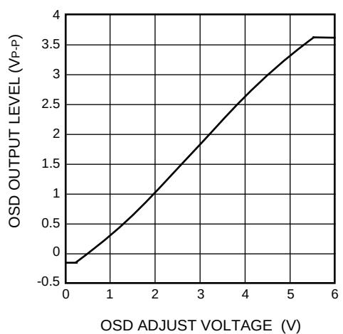
OSD ADJUST VOLTAGE VS. OSD OUTPUT LEVEL
