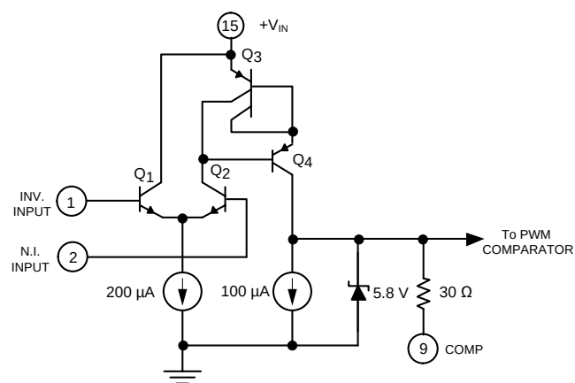
Figure 5 • Error Amplifier
