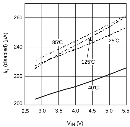
Figure 11. I_Q (disabled) vs V_{IN} and Temperature, E_N = 0 V
