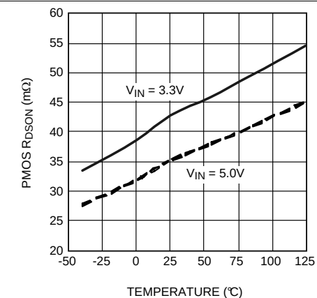
Figure 6. PMOS R_{DS(ON)} vs Temperature
