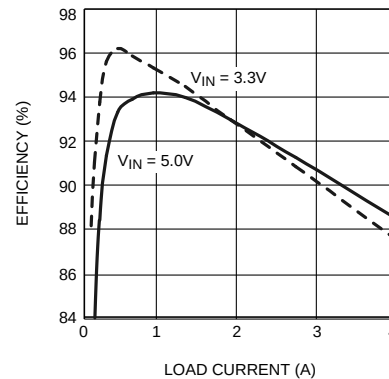
Figure 31. LM2854 500-kHz Efficiency vs I_{OUT} V_{OUT} = 1.8\text{ V} , L_O = 1.5\text{ }\mu\text{H} , 9.7-m \Omega DCR
