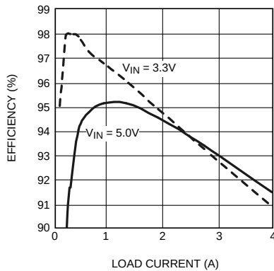
Figure 28. LM2854 500-kHz Efficiency vs I_{OUT} V_{OUT} = 2.5\text{ V} , L_O = 2.2\text{ }\mu\text{H} , 16-m \Omega DCR
