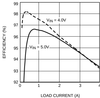
Figure 30. LM2854 500-kHz Efficiency vs I_{OUT} V_{OUT} = 3.3\text{ V} , L_O = 1.5\text{ }\mu\text{H} , 9.7-m \Omega DCR
