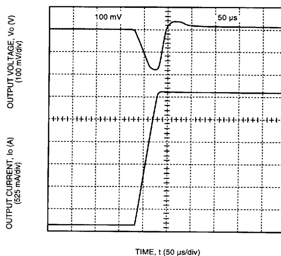
Figure 7. Typical FE150B Transient Response to Step Increase in Load from 50% to 75% of Full Load at Room Temperature and 48 V Input (Waveform Averaged to Eliminate Ripple Component.)
