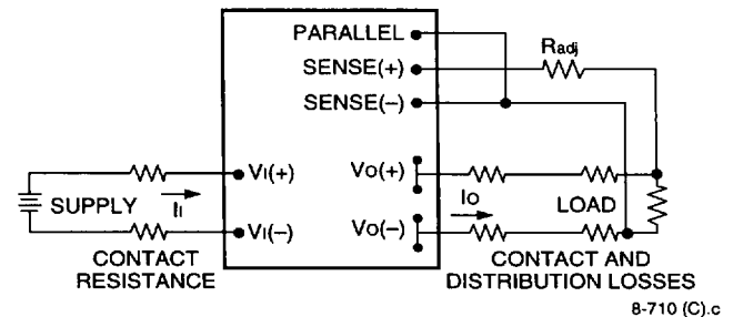
Figure 16. Circuit Configuration to Adjust Output Voltage
