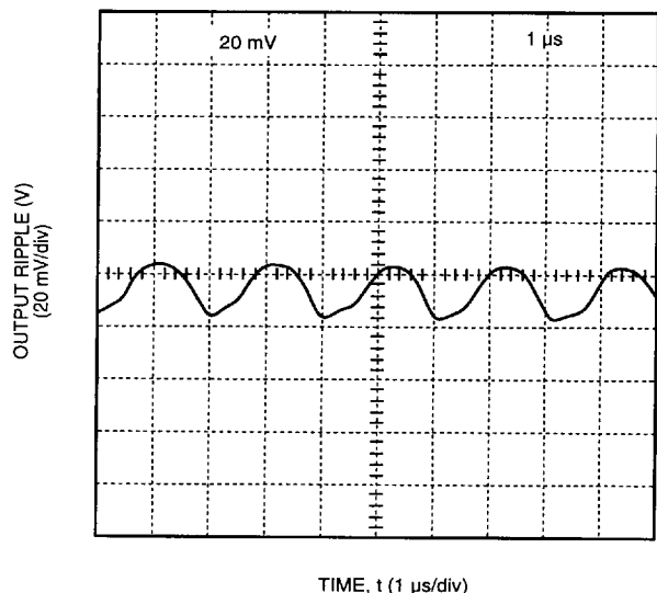
Figure 5. Typical FE150B Output Ripple Voltage at Room Temperature, 48 V Input, and 12.5 A Output
