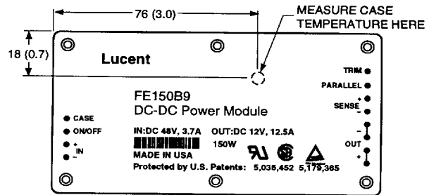
Figure 18. Case Temperature Measurement Location
