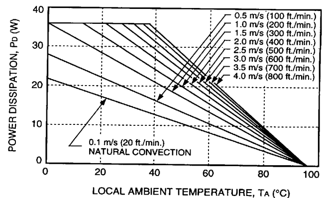
Figure 19. Power Derating vs. Local Ambient Temperature and Air Velocity
