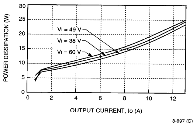
Figure 22. FE150B Power Dissipation as Heat vs. Output Current
