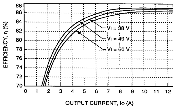
Figure 4. Typical FE150B Efficiency vs. Output Current at Room Temperature
