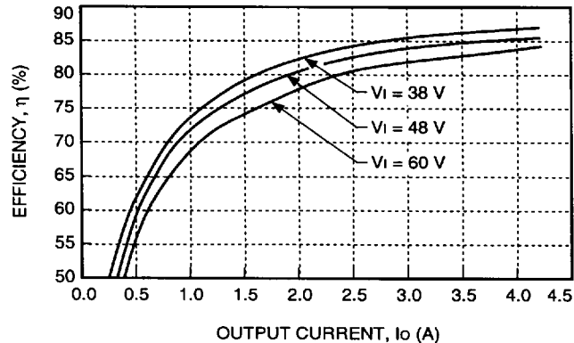
Figure 3. Typical FE050B Efficiency vs. Output Current at Room Temperature
