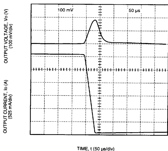
Figure 6. Typical FE150B Transient Response to Step Decrease in Load from 50% to 25% of Full Load at Room Temperature and 48 V Input (Waveform Averaged to Eliminate Ripple Component.)
