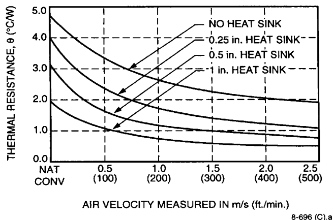
Figure 20. Heat Sink Resistance Curves; Fins Oriented Along Width
