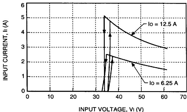
Figure 1. Typical FE150B Input Characteristics at Room Temperature
