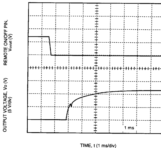
Figure 8. Typical FE150B Start-Up Transient at Room Temperature, 48 V Input, and 12.5 A Output
