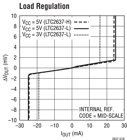
LTC2637
