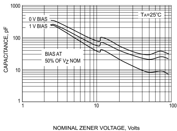
TYPICAL CAPACITANCE
