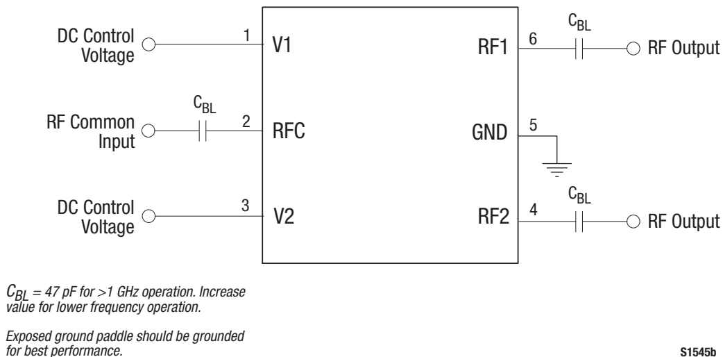
Figure 7. SKY13370-374LF Evaluation Board Schematic
