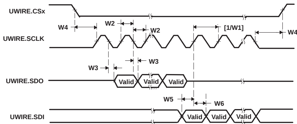
Figure 5–35. MICROWIRE Timings
