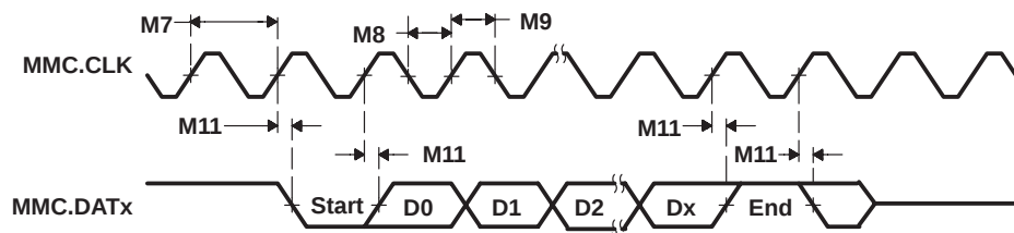
Figure 5–31. MMC/SD Host Write Timings
