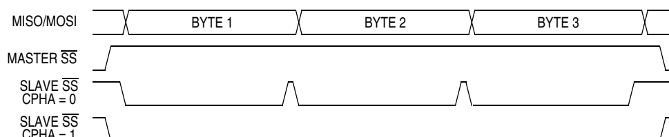
Figure 16-6. CPHA/\overline{SS} Timing
